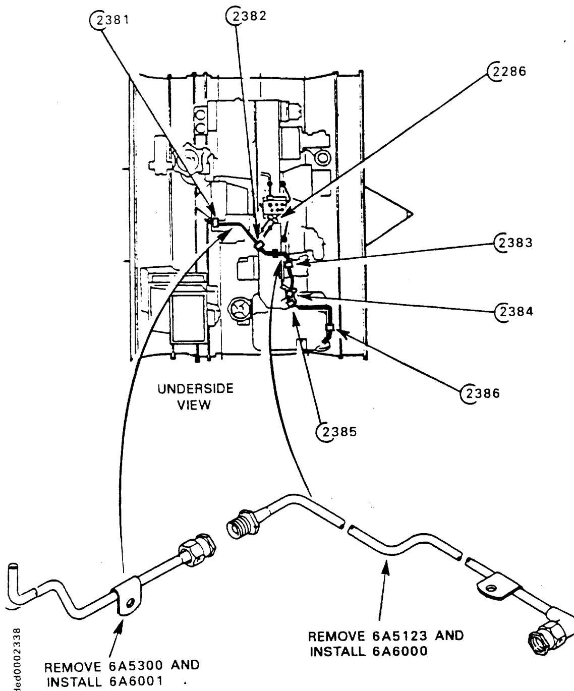
Location of tubes and clipping points Fig.1 (Sheet 1 of 2)
