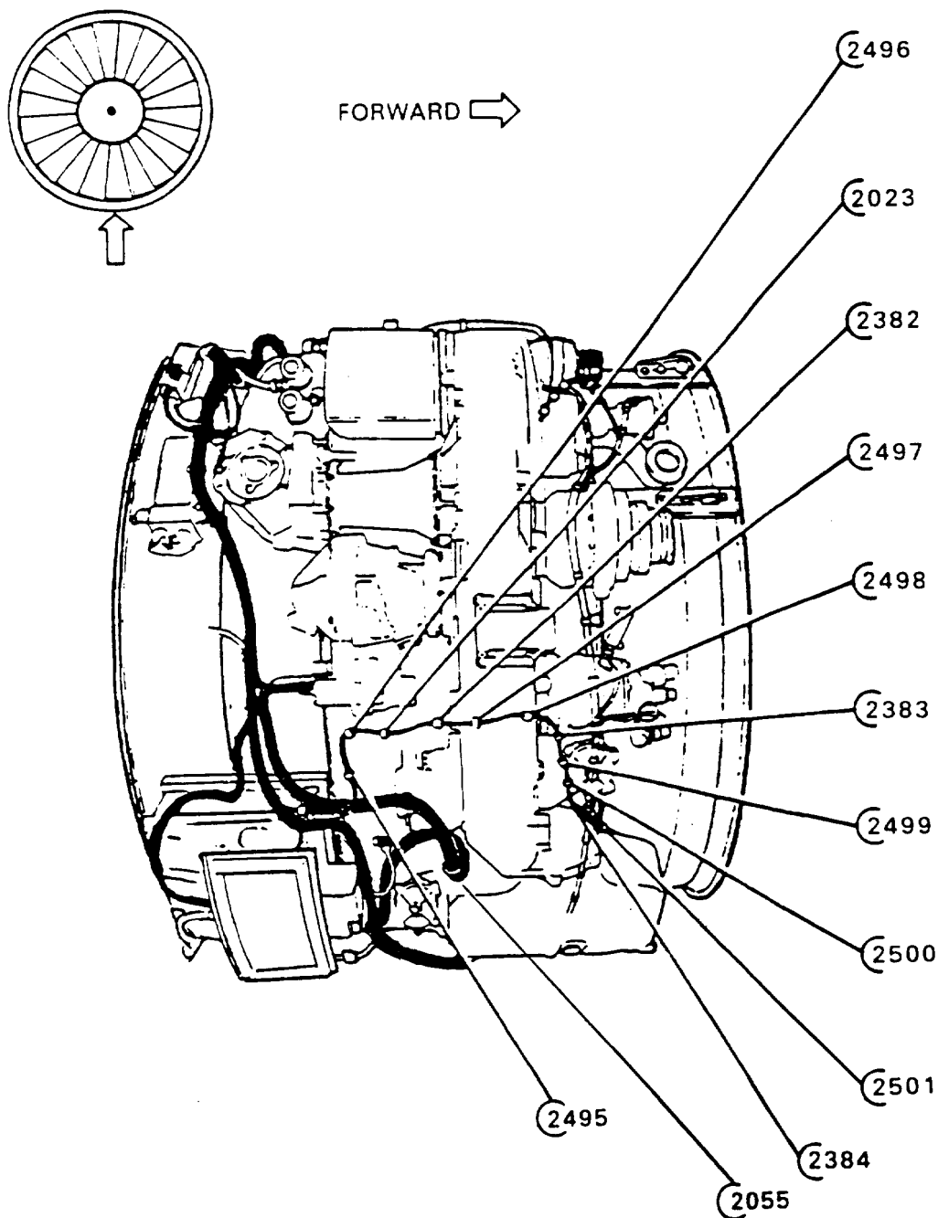
Location of tubes and clipping points Fig.1 (Sheet 2 of 2)
