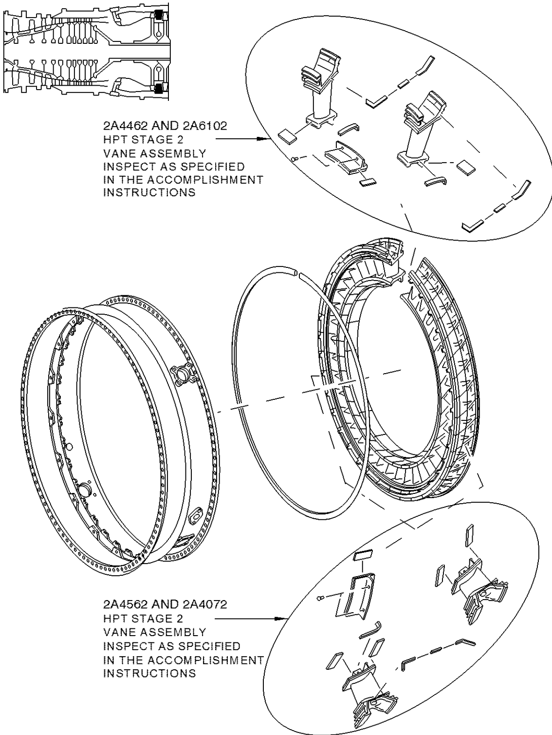
LOCATION OF THE HPT STAGE 2 VANE ASSEMBLY 72-45-24 FIGURE 1
