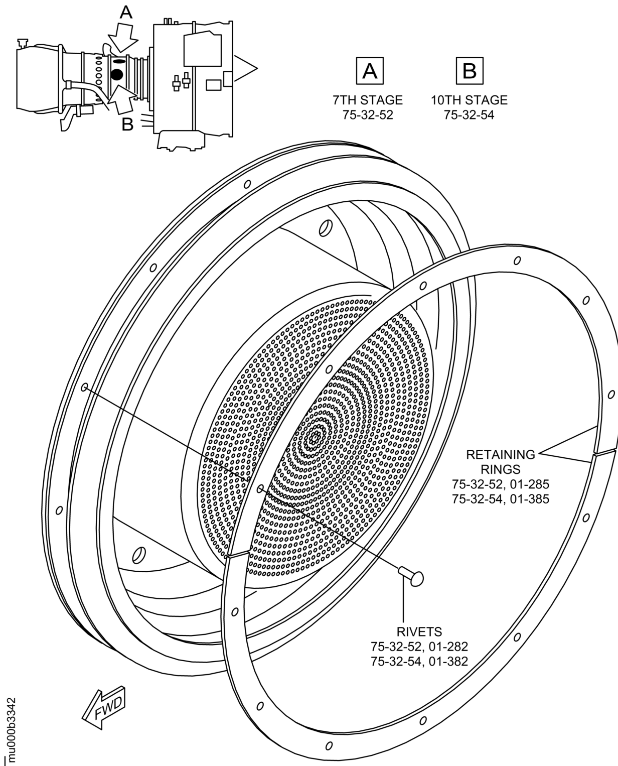
LOCATION OF THE SILENCER ON THE 7TH AND 10TH STAGE HPC BLEED VALVES FIGURE 1
