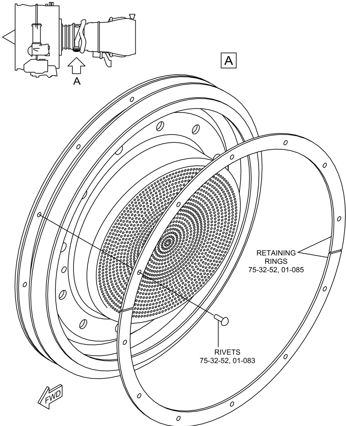
LOCATION OF THE SILENCER ON THE 7TH STAGE HPC BLEED VALVE FIGURE 2
